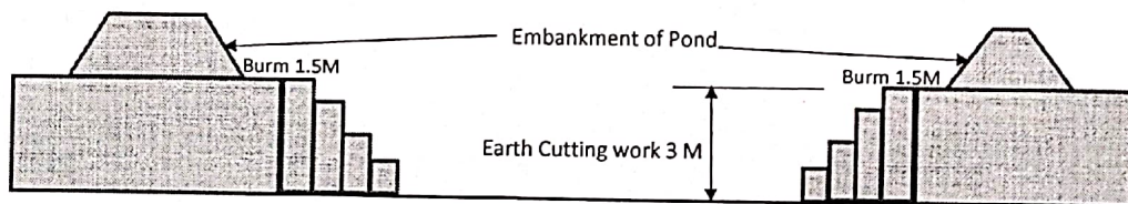
Cross Section of Pond
